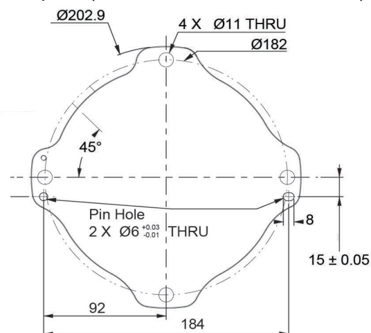
Footprint (TM6S/12S/14S/20S Models)
