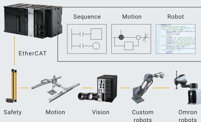
Robot integrated CPU unit NJ501-R
